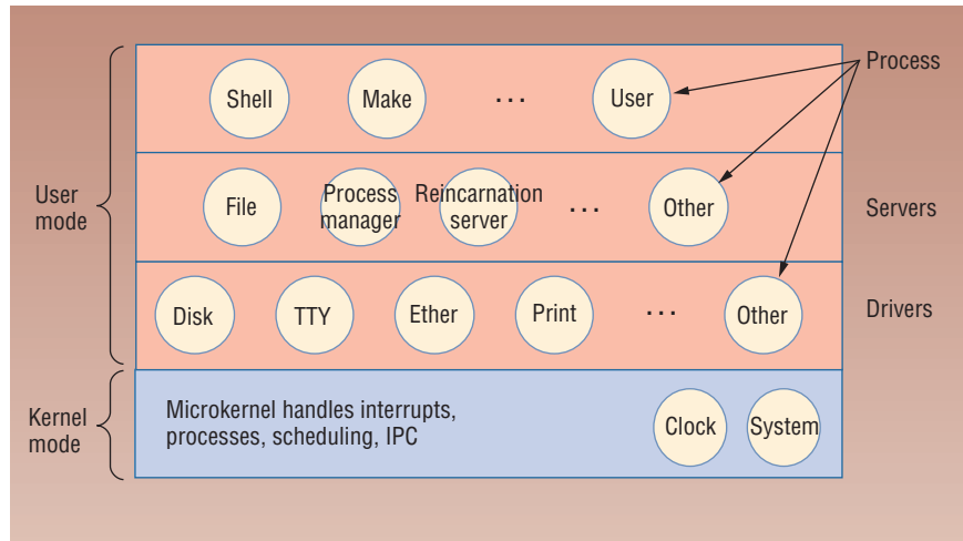
Figure 3. The Minix 3 architecture. The microkernel handles interrupts, provides the basic mechanisms for process management, implements interprocess communication, and performs process scheduling.
